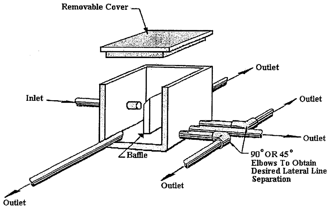
Figure 7 Distribution Box
