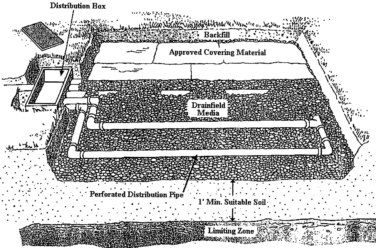
Figure 3 Conventional Absorption Bed
